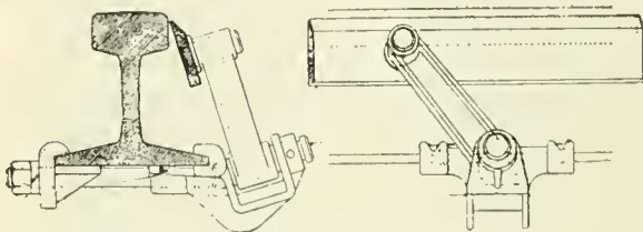
DETECTOR BAR, WHICH PREVENTS SWITCH BEING THROWN WITH ENGINE OR CARS STANDING OVER IT.
